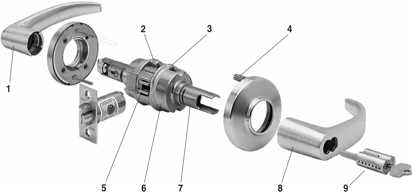
9K – EXPLODED
