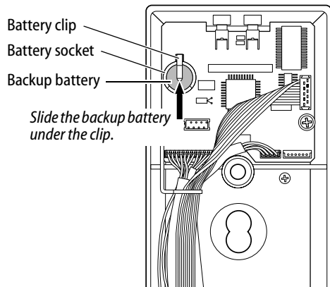
Figure 2 Installing the backup battery
