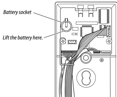
Figure 1 Removing the backup battery
