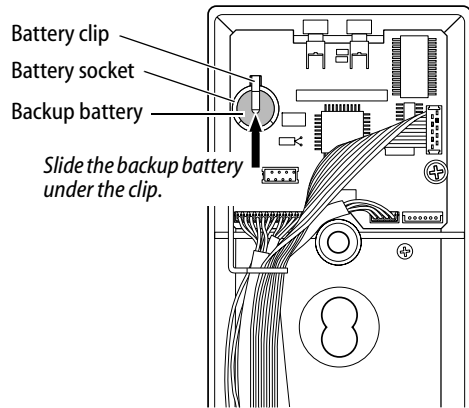
Figure 5 Installing the backup battery
