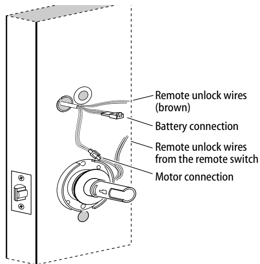
Figure 3 Making the remote unlock connection (cylindrical installation shown)
