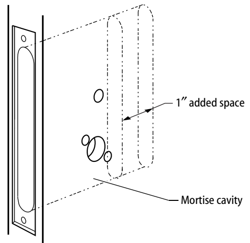
Figure 2 Extending the mortise cavity for wire connections
