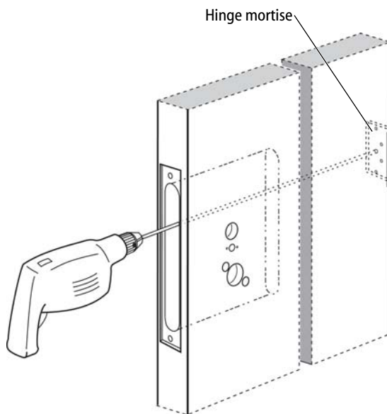
Figure 3 Drilling the wire channel through the door
