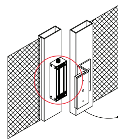
Single swing gate installation
