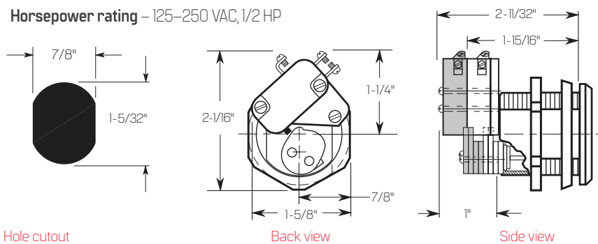
Hole cutout
