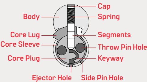
Cormax Core – Cross Section
